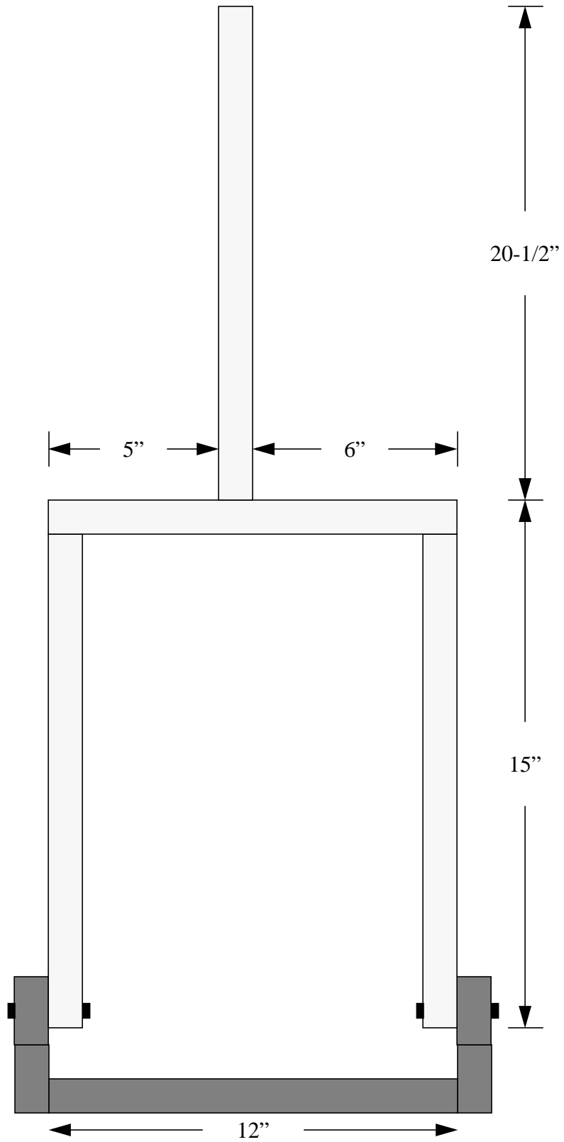
(Back View)
